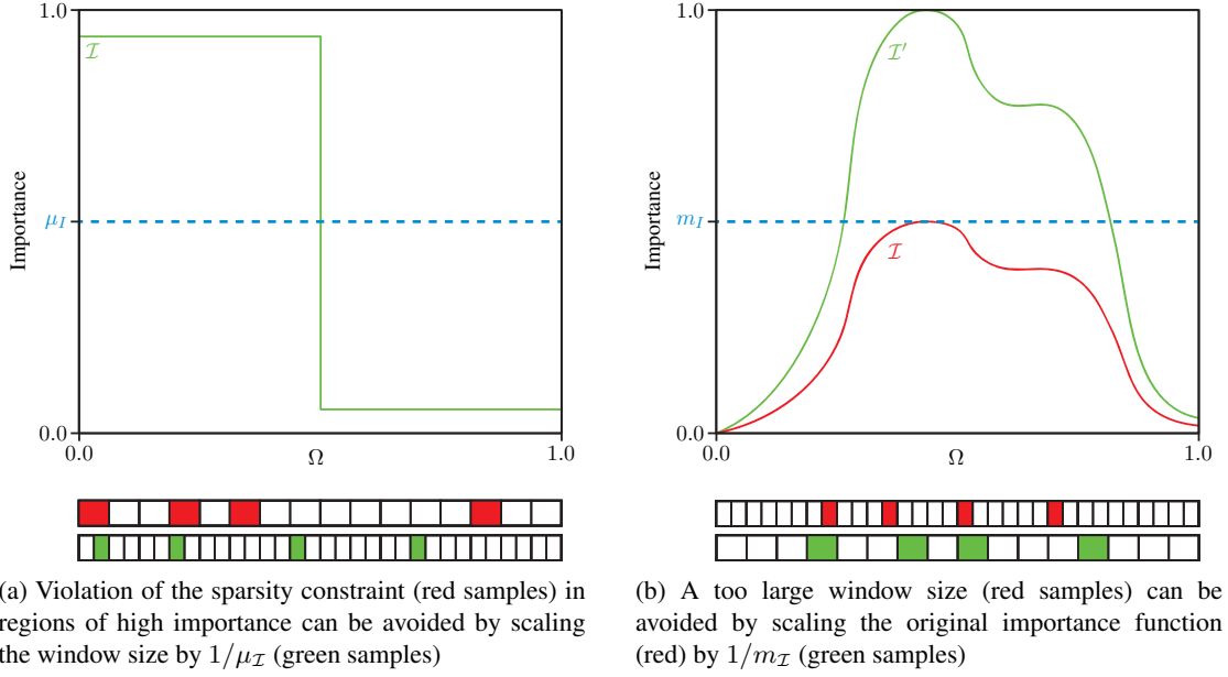
Figure 4.3: Influence of average and maximum importance on the window size
