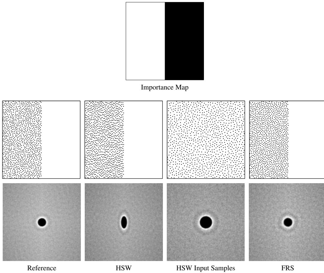
Figure 6.12: Adaptive sampling with a highly anisotropic importance map
