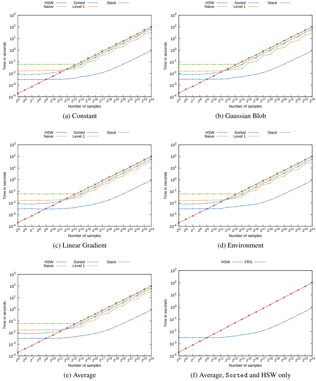
Figure 6.13: Time consumption of the FRS CPU implementations Naive, Sorted, Level 1 and Stack compared to HSW for different importance maps
