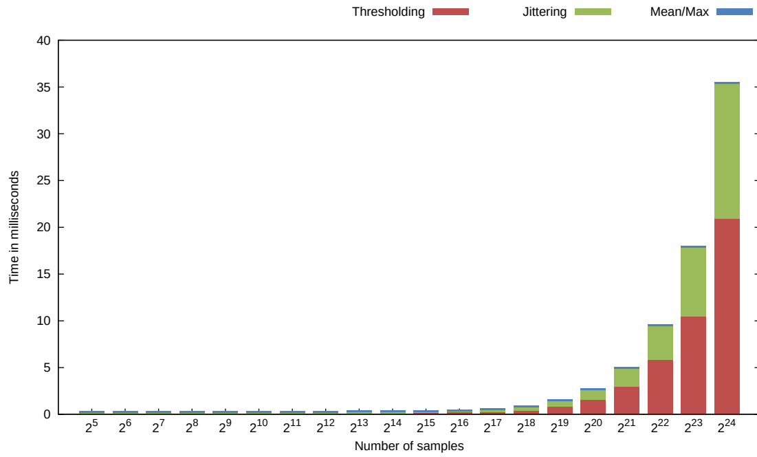
(a) Jittered Sorted
