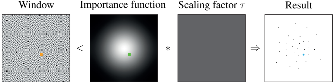
Figure 4.2: Illustration of the thresholding inequation of Forced Random Sampling
